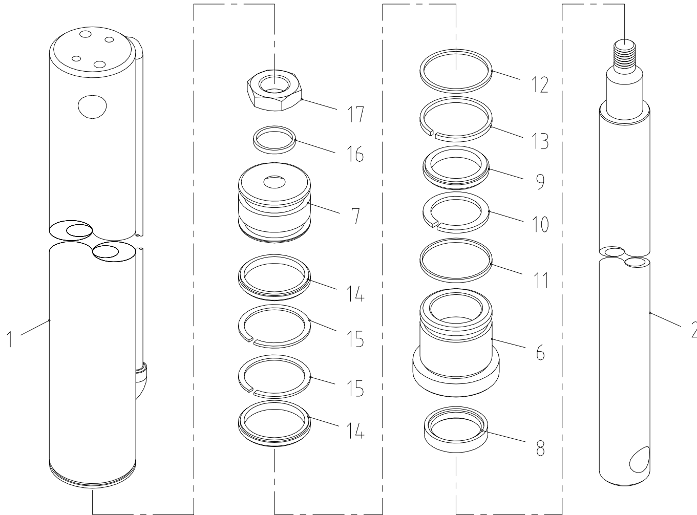
Fig. 4-1 SCS263 JACK CYL' ASS'Y
