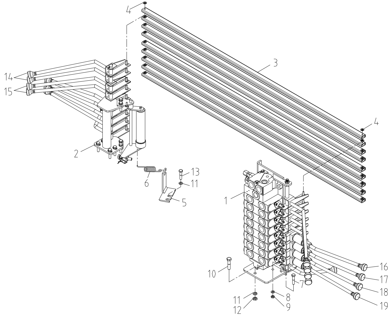
Fig. 3-4 SCS263 OPERATION MAIN ASS'Y
