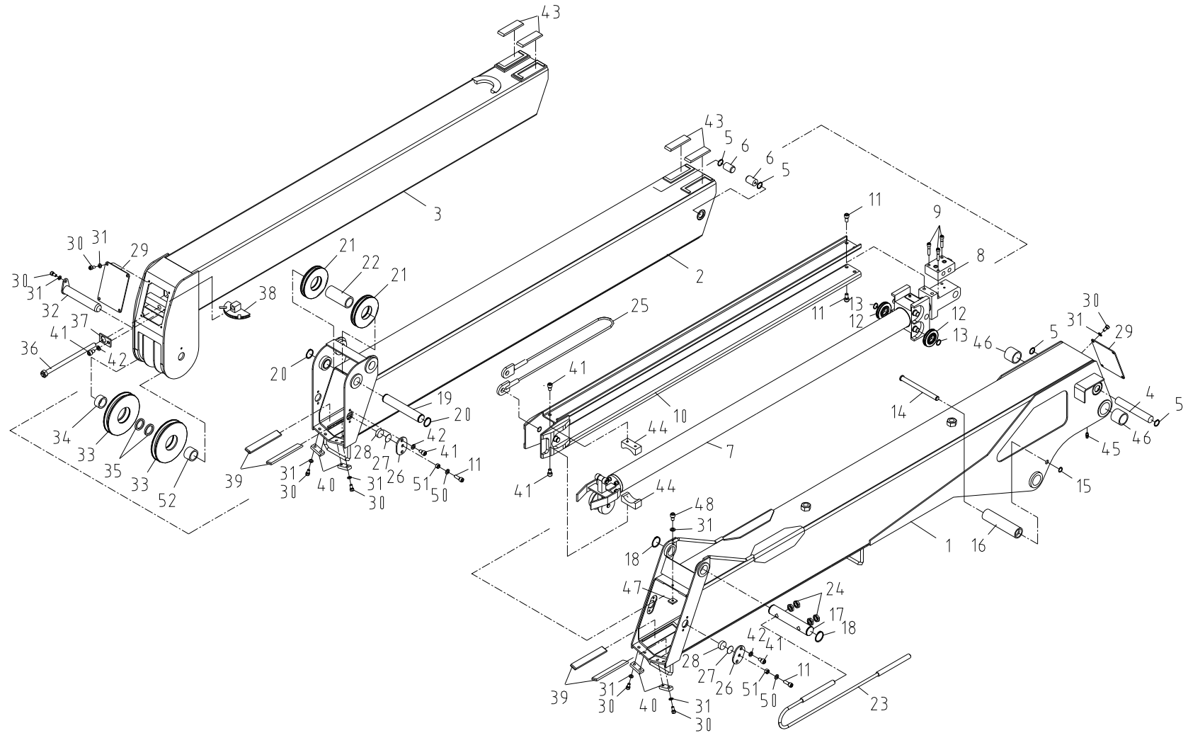
Fig. 1 SCS263 BOOM ASS'Y
