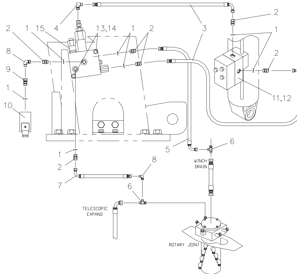
Fig. 5-7 SCS263 LOAD LIMMIT PIPING
