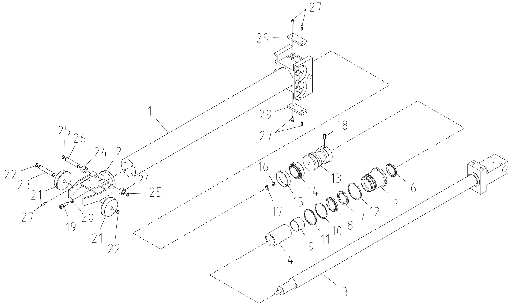
Fig. 1-1 SCS263 TELE' CYL' ASS'Y
